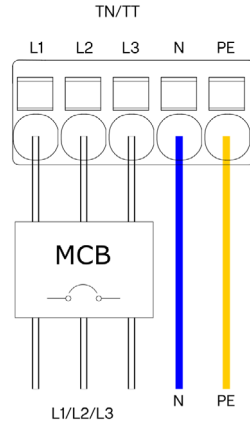
3 phase connection
